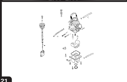
Carburador / Carburetor GAS GAS EC/MC/SM 2006
