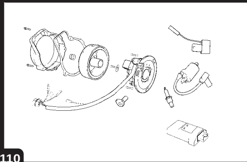
Encendido / Ignition GAS GAS EC/MC/SM 2006
