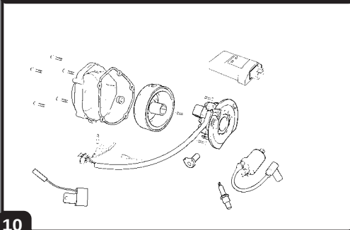
Encendido / Ignition GAS GAS EC/MC/SM 2006
