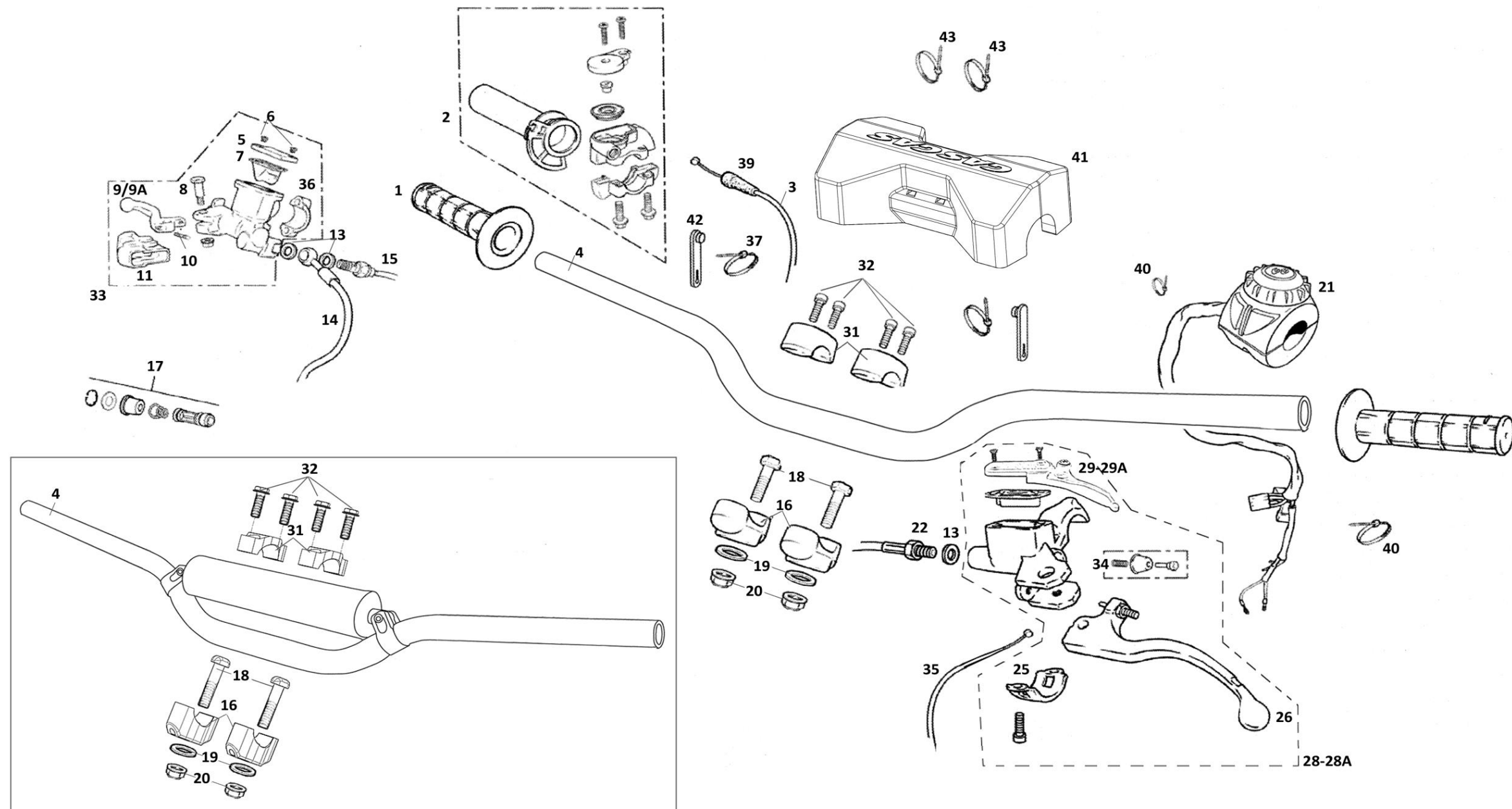
MANILLAR RACING / RACING HANDLEBAR
