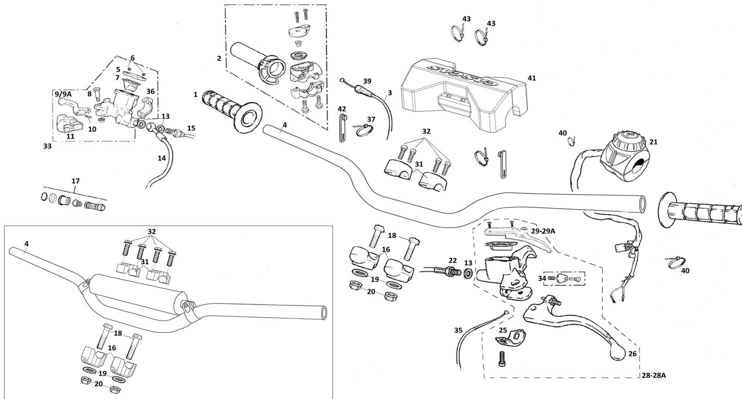
MANILLAR RACING / RACING HANDLEBAR
