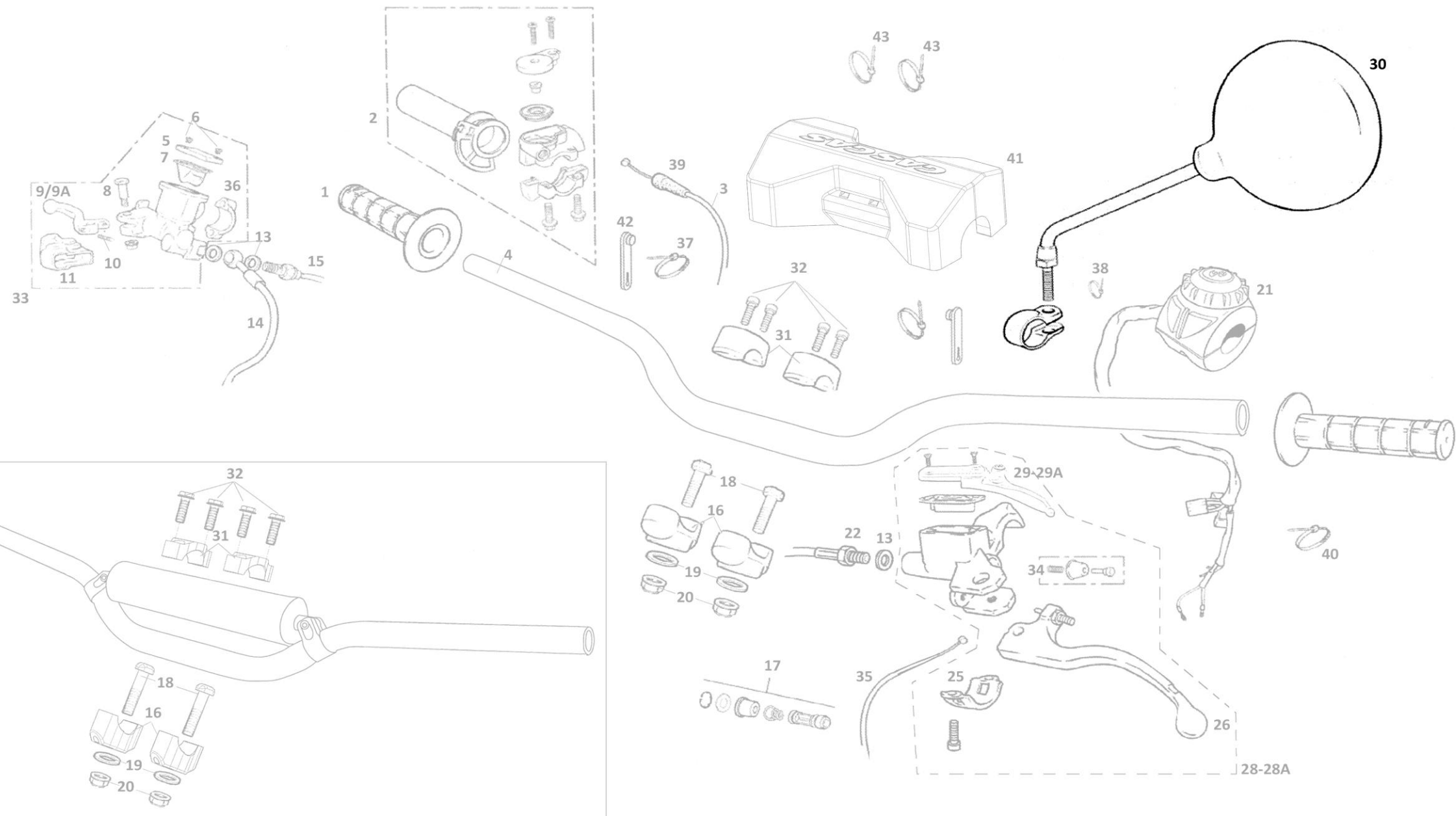
MANILLAR RACING / RACING HANDLEBAR
