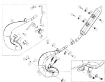
Escape
